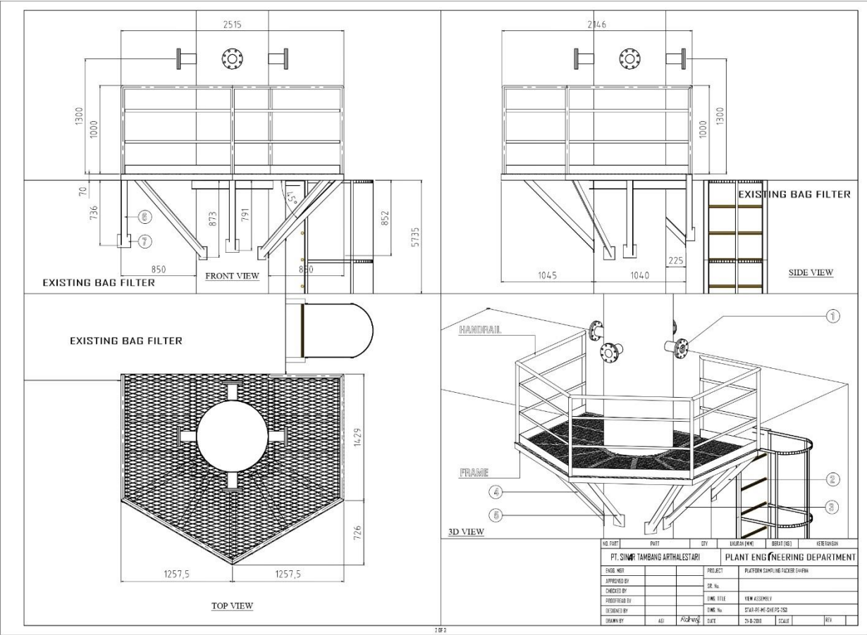
Gambar 69. Sarana dan Prasarana Pengambilan Sampel di Cerobong Cement Packer
